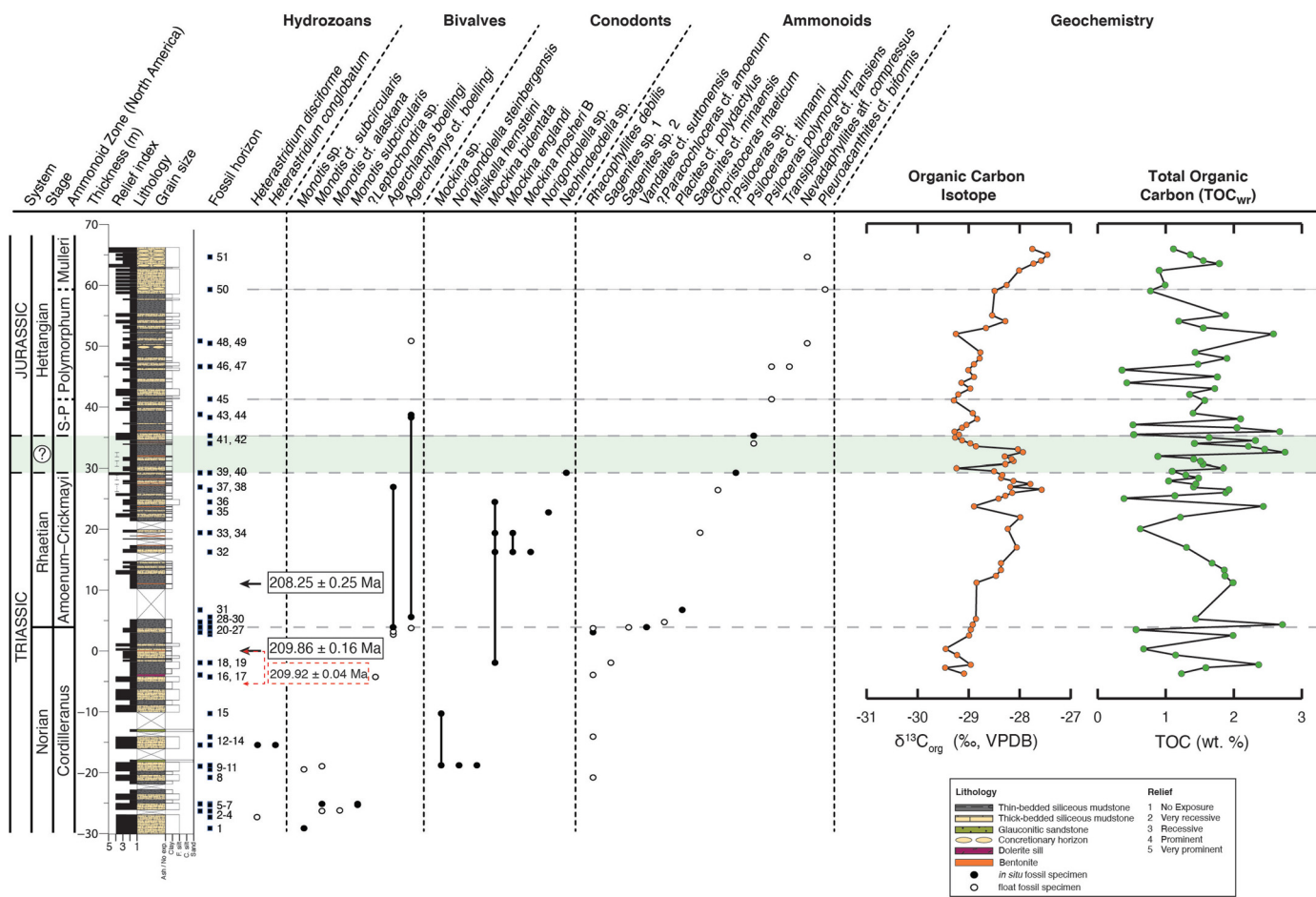
Fig. 3. Compilation data from the Grotto Creek section, Alaska (base at 61°30'13.23''N, 142°26'31.51''W) showing combined lithological, paleontological, and geochemical results. Note: Shaded area represents the suspected TJB interval; vertical hash marks indicate intervals of poor exposure; Dashed red box and corresponding dashed red arrows represent suspected interval of dated ash by Witmer (2007), solid black arrows and boxes denote new dates in this study; filled circles are in situ fossil occurrences, open circles are float specimens; TOC wr denotes Total Organic Carbon measured from whole rock; Sp. = Spelae; Pac. = Pacificum; exp. = exposure.
