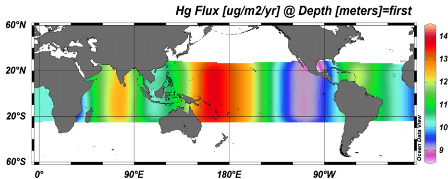
Fig. 2. Annual mercury deposition (wet plus dry, including Hg(0); \mu\text{g m}^{-2} \text{yr}^{-1} ) over the tropical oceans simulated using GEOS-Chem. Deposition shown here is averaged over tropical latitudes (24°N to 24°S).
