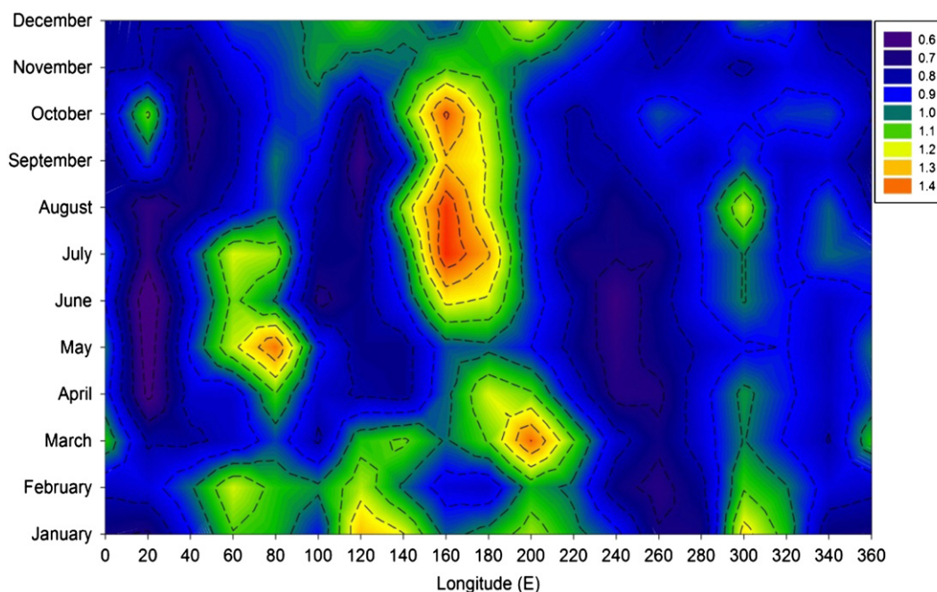
Fig. 3. The seasonal variability in total mercury 1 deposition (wet plus dry including Hg(0); \mu\text{g m}^{-2} \text{month}^{-1} ) across longitude simulated using GEOS-Chem.
