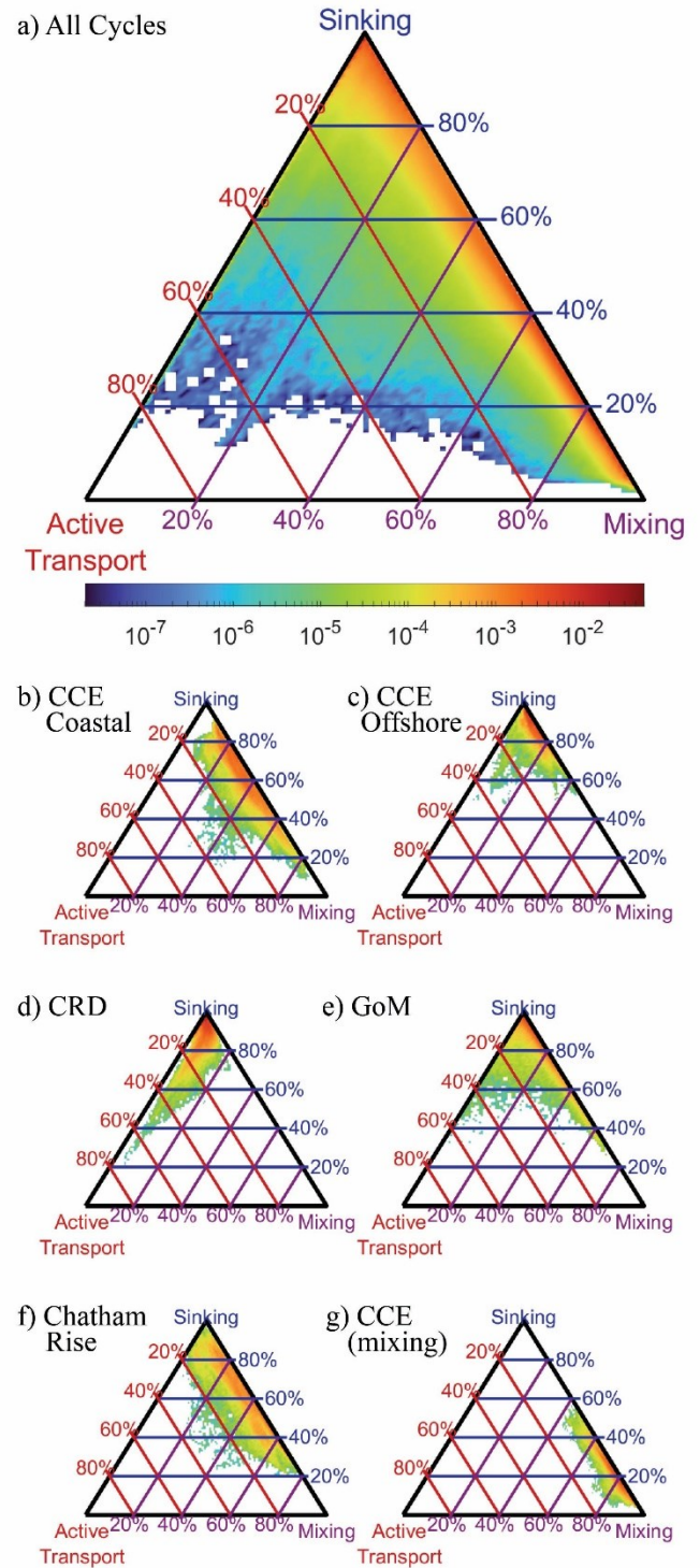
Figure 9 – Triangle diagrams showing the proportion of export due to each biological carbon pump pathway at the base of the euphotic zone. Locations near the upper apex of the triangle indicate dominance by sinking particles, locations near the bottom left indicate dominance by active transport, locations near the bottom right show dominance by mixing. Colors represent the proportion of total model simulations with export patterns falling within a specific proportion of different export pathways. Lines indicated contours showing a constant proportion of one BCP pathway (i.e., red lines are constant proportions of active transport, blue lines are constant proportions of gravitational flux, and purple lines are constant proportions of mixing flux). a) results for all simulations, b) results for a typical CCE coastal site (1604-3), c) typical CCE oligotrophic site (1408-5), d) typical Costa Rica Dome site (CRD-1), e) typical Gulf of Mexico site (GoM-5), f) typical Chatham Rise site (Salp-5), g) example of a CCE site (0605-3) dominated by mixing flux.
