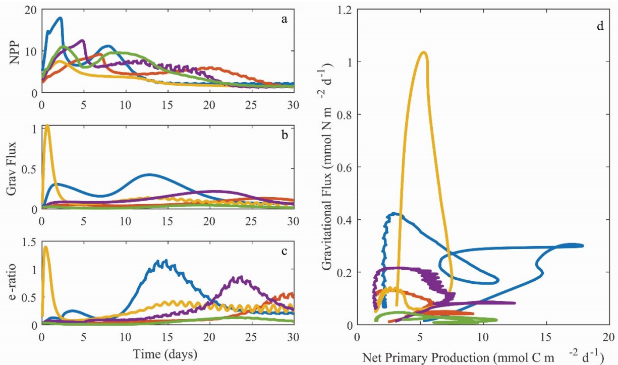
Figure 12 – Temporal variability in net primary production (a, \text{mmol C m}^{-2} \text{ d}^{-1} ), gravitational flux (b, \text{mmol N m}^{-2} \text{ d}^{-1} ), and export efficiency (c, unitless with a C:N conversion ratio of 106:16 mol:mol), along with a phase-space plot depicting the same data (d). All plots are from Lagrangian experiment 1604-3 (CCE upwelling region). Different colors are for simulations with ensemble parameter sets 2 \times 10^5 , 4 \times 10^5 , 6 \times 10^5 , 8 \times 10^5 , or 10^6 .
