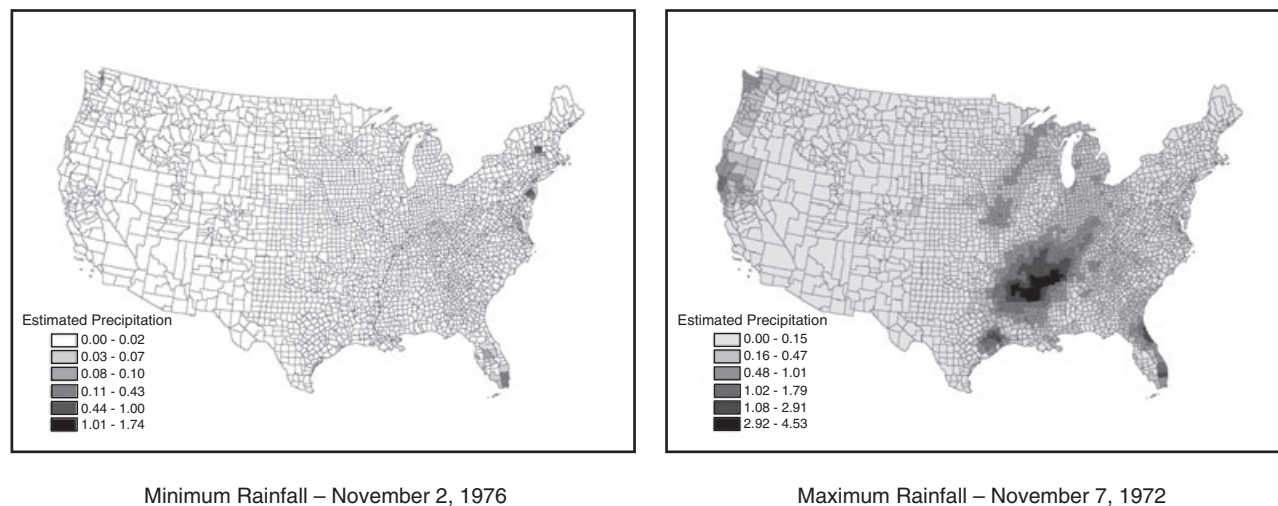
FIGURE 1 Maps of Election Days with Minimum and Maximum Rainfall
